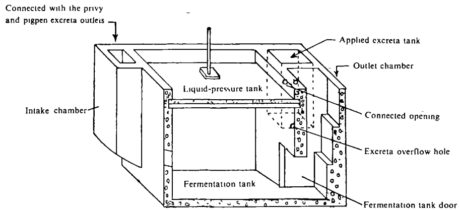
Enclosed three-stage biogas plant with applied excreta tank (from 4504).
