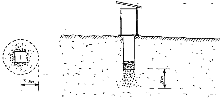
Movement of pollution in dry soil from the pit privy (from 2108).
