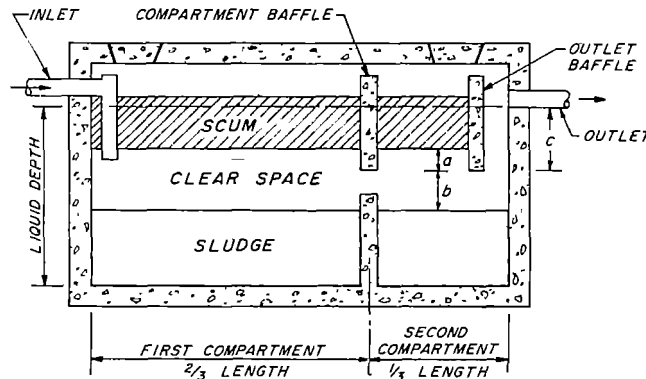
Two-compartment septic tank: a, scum clear space (75 mm minimum); b, sludge clear space (300 mm minimum); c = 40% of liquid depth.
