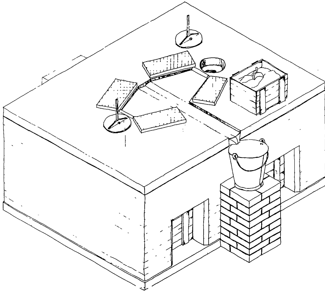
The Vietnamese double vault.
