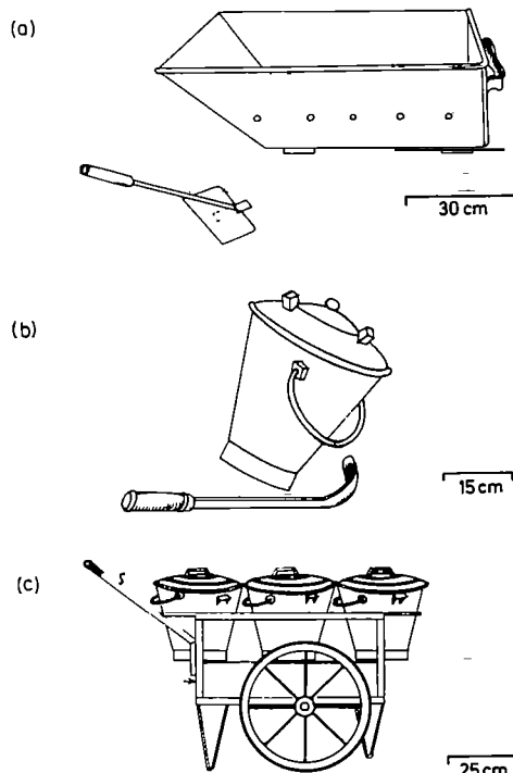
(a) Night-soil container (made from 24-gauge galvanized iron sheet) and scraper. (b) Night-soil bucket and scraper. (c) Wheelbarrow for three or six buckets (from 3116). (Designs by Department of Social Welfare, Ahmadabad.)
