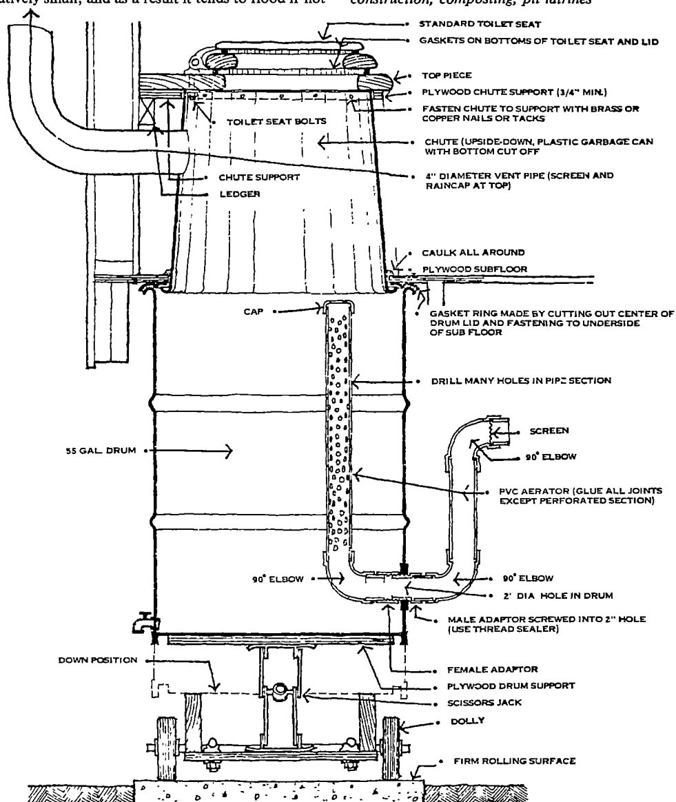
Matson drum privy (from 2135).
