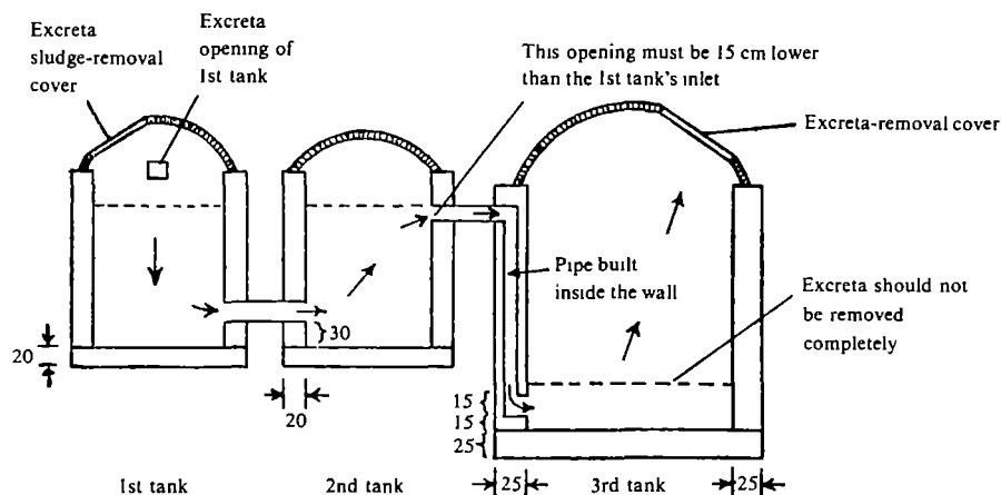
The Chinese three-tank toilet (from 2303).
