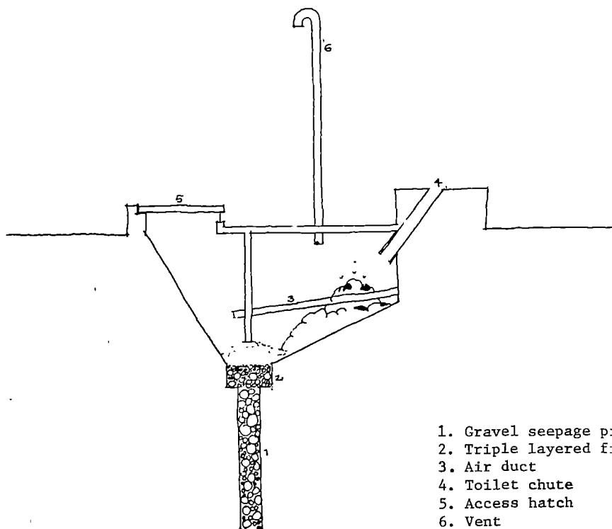
The biopit composting toilet (from 2219).
