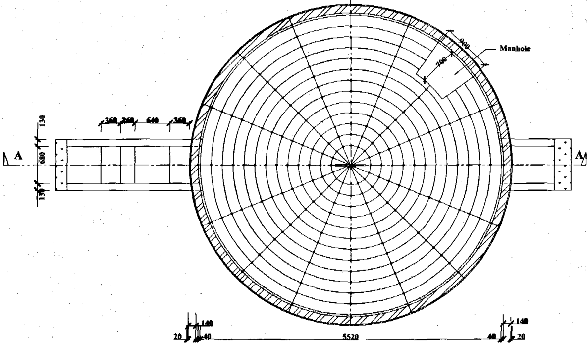
PLAN (mm)
