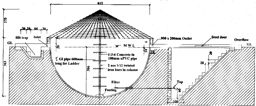
SECTION A - A (cm)
