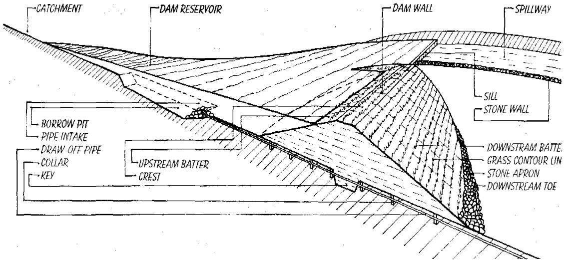
Cut-through section of a three-dimensional sketch of a dam wall.
