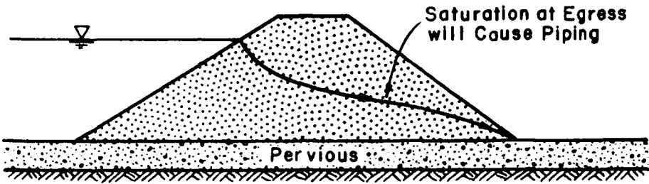
(b) Pervious Foundation without Drainage
