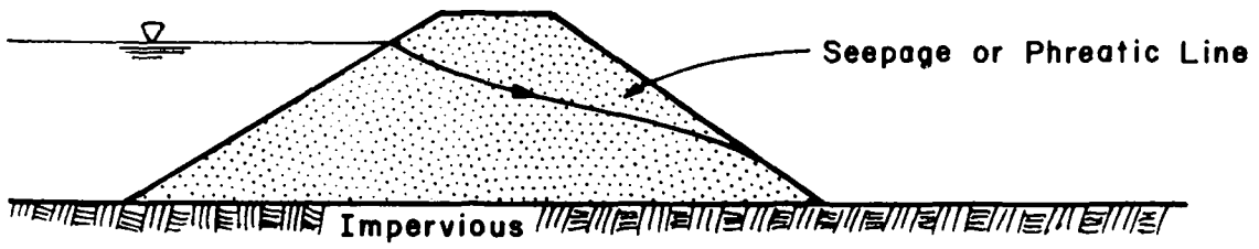
(a) Impervious Foundation without Drainage
