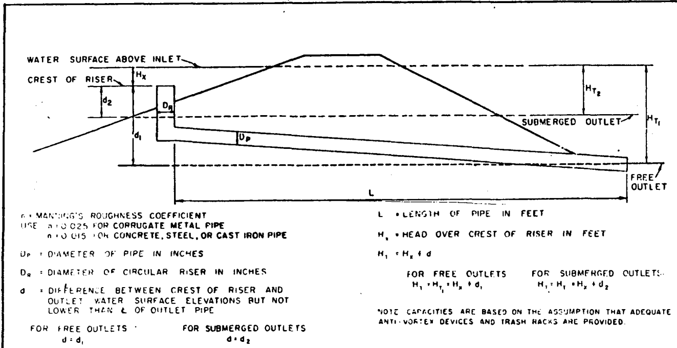
FIGURE 20 - TYPICAL PIPE SPILLWAY DESIGN CHART (U.S. Soil Conservation Service, 1969)
