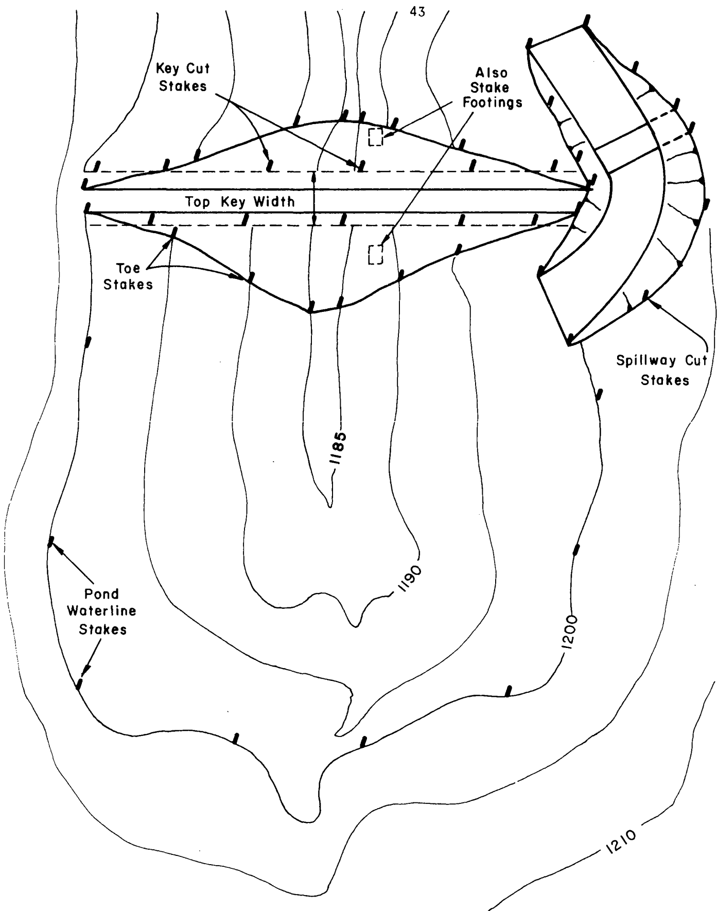
FIGURE 27 - STAKING LAYOUT
