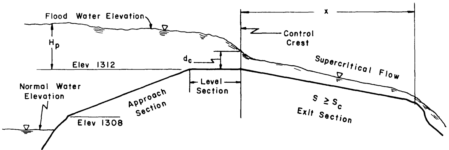
(b) Profile Along ℄ of Spillway
