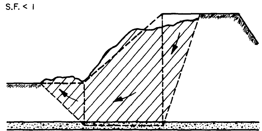
(b) TRANSLATORY SLIDE
