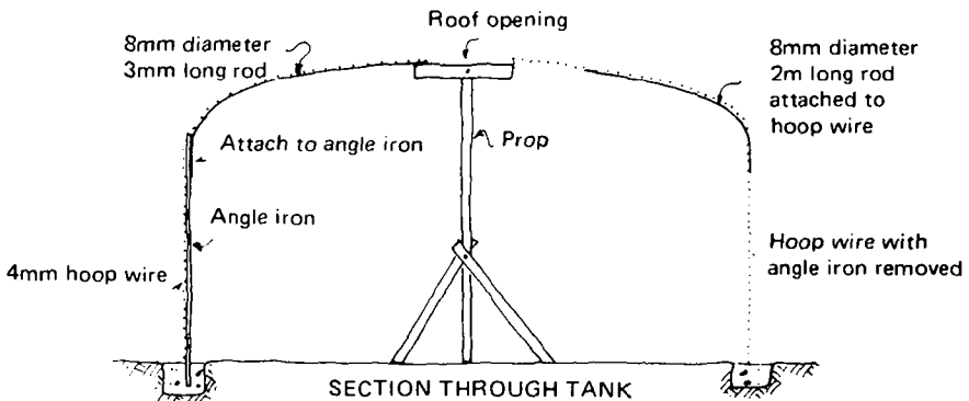
Fig.38 Building the roof
