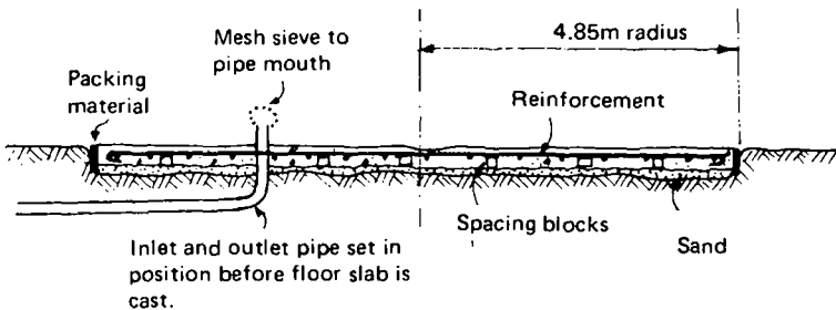
Fig.25 Casting the floor slab
