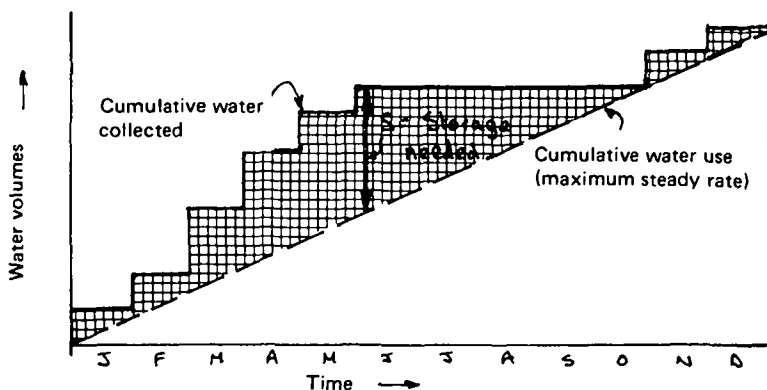
Fig. 42 Estimating tank size
