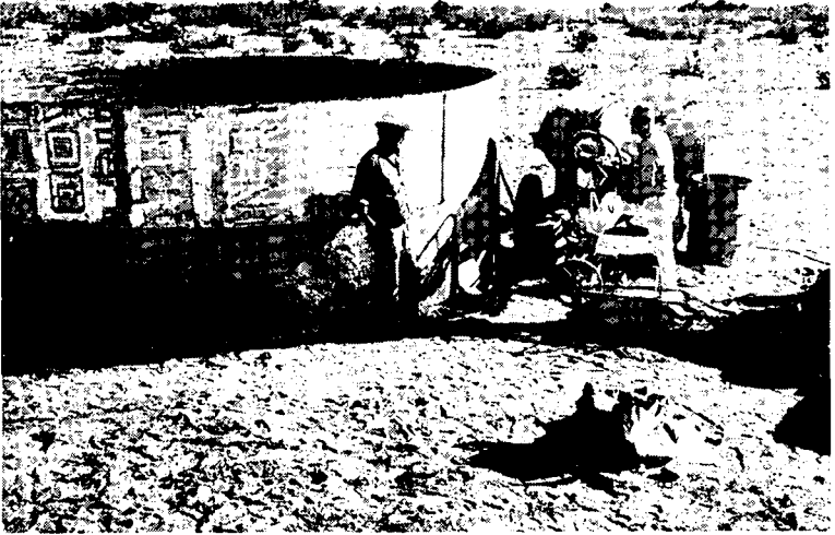
10.1 Cheap shuttering from flattened oil drums
