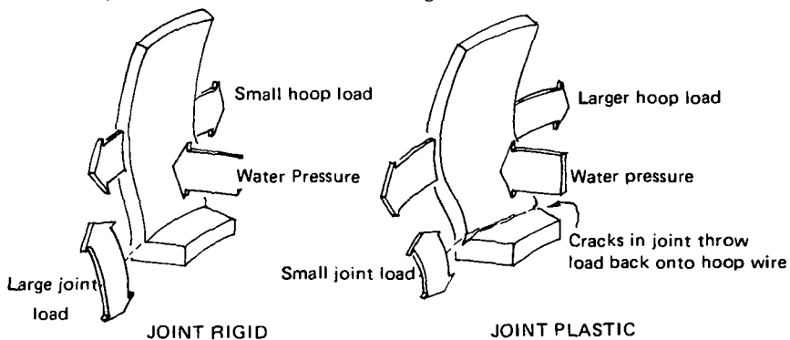
Fig. 9 How the loads are taken
