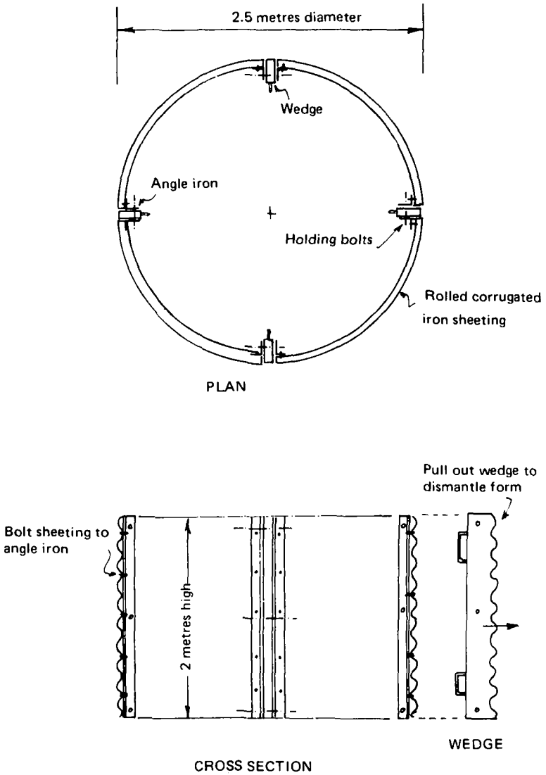
Fig.18 Standard formwork to make 10m 3 tank
