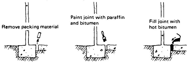
Fig.27 Making the expansion joint
