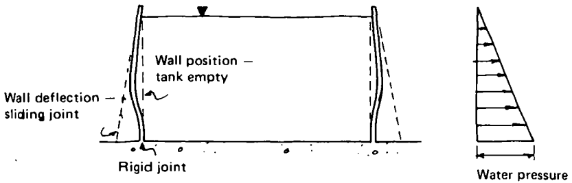
Fig. 8 Walls joined with floor
