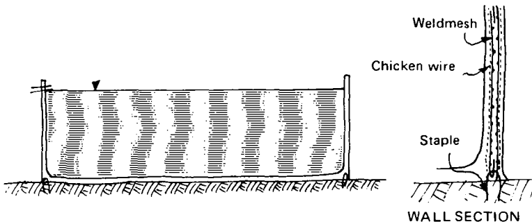
Fig.39 Construction of 150m 3 tank, USA
