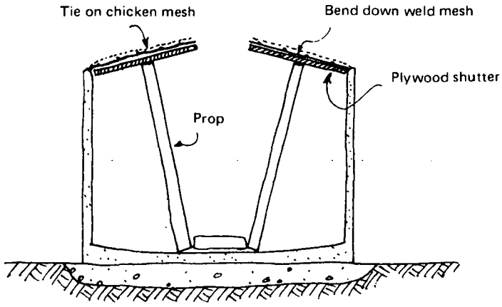
Fig.35 Making the roof
