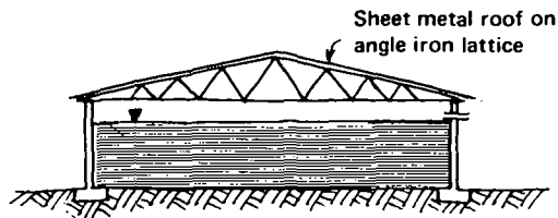
Fig.12 Roof for larger tank
