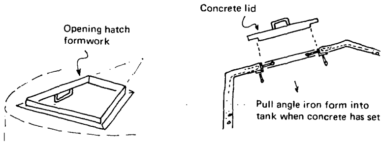
Fig.32 Making the access hatch
