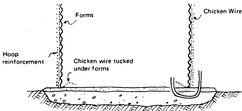
Fig.21 Erect formwork and wind on reinforcing wire
