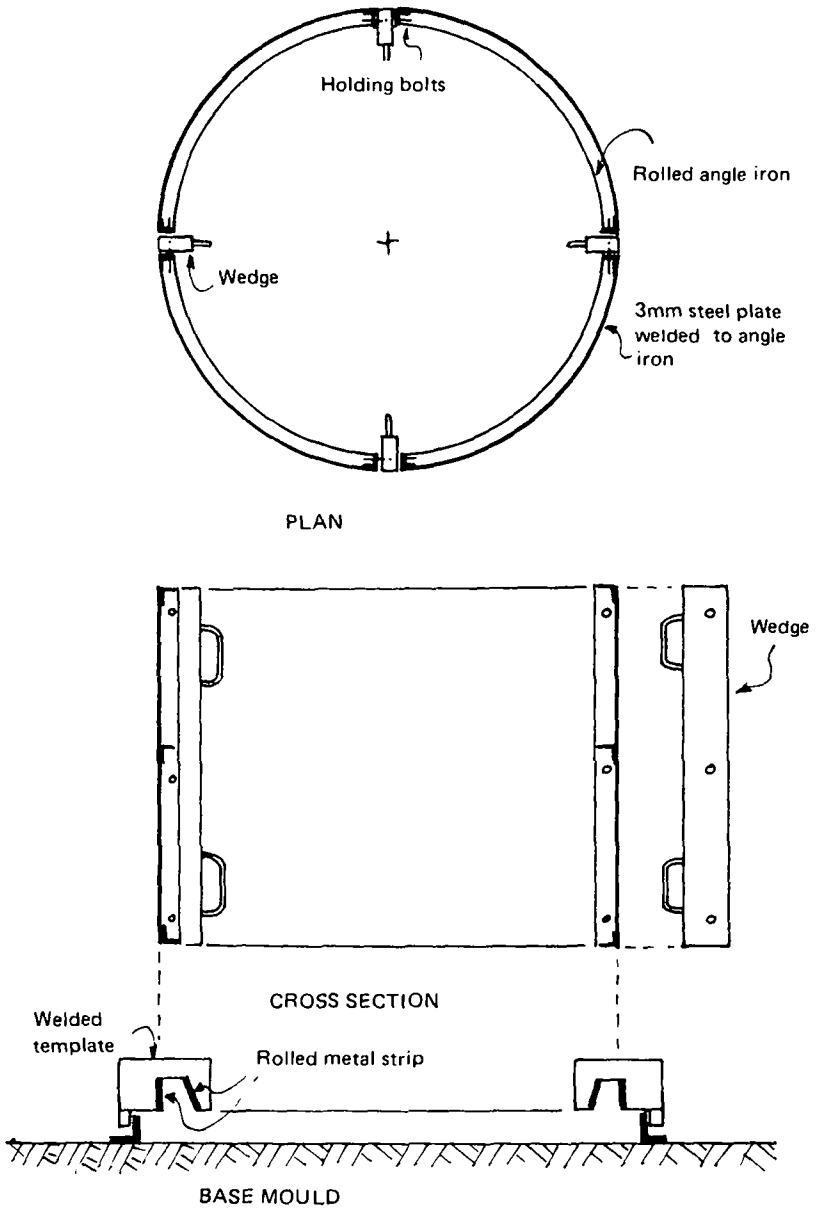
Fig 28 Commercial tank formwork
