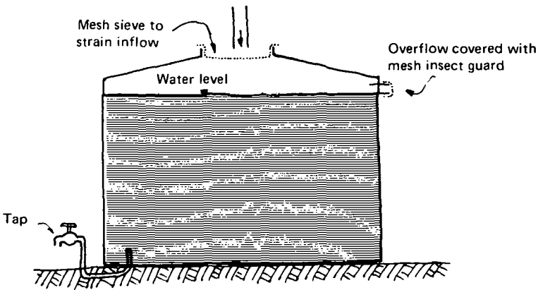
Fig.2 Protecting the tank from further contamination
