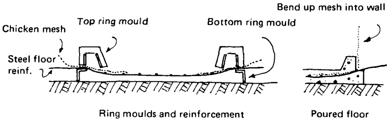
Fig.29 Casting the base slab
