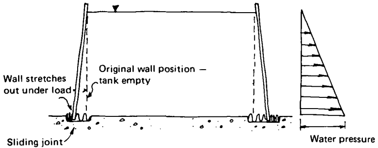
Fig. 7 Walls free to move – exaggerated wall deflection
