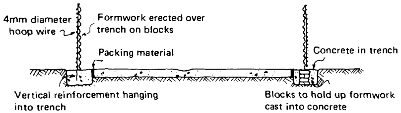
Fig.26 Assembling the formwork
