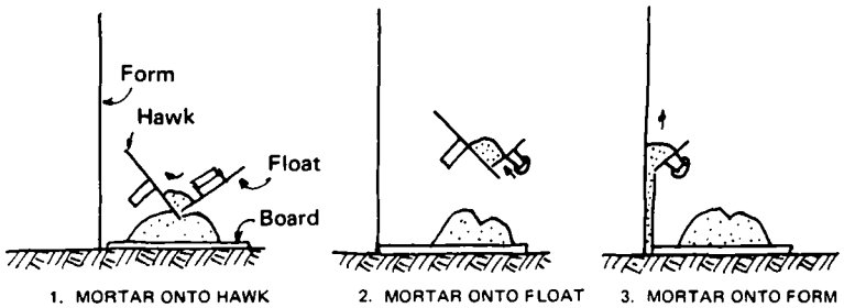
Fig.17 Trowelling the mortar onto the formwork
