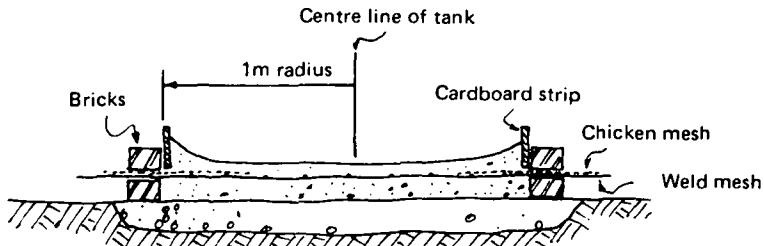
Fig.33 Making the base of the tank
