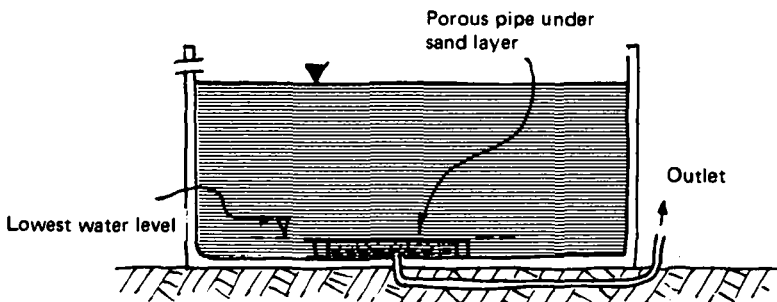
Fig.14 Slow sand filter in tank over outlet
