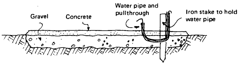
Fig.20 Foundation of tank
