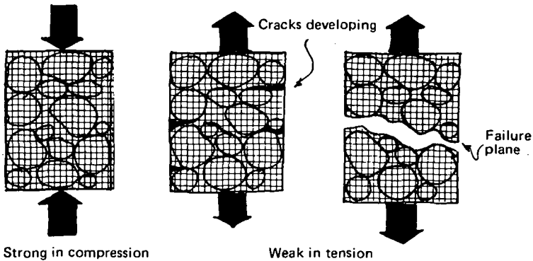
Fig. 3 The mortar under load
