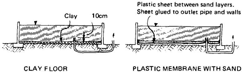
Fig.10 Alternative floors
