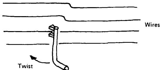
Fig.16 Tool for tightening wires
