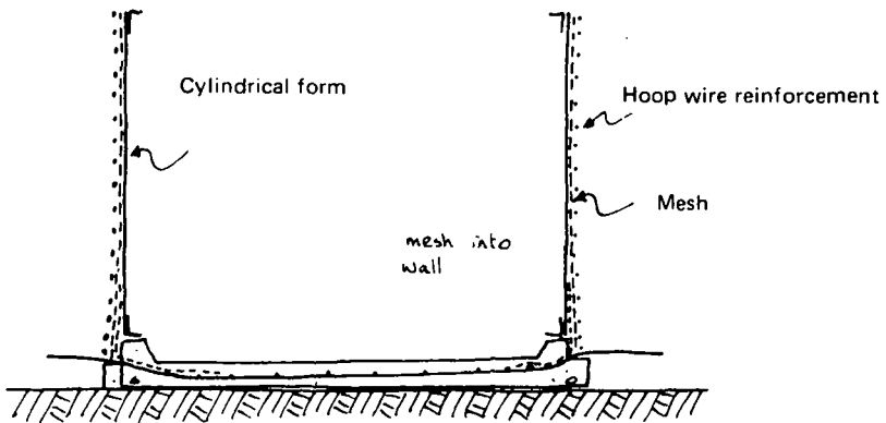
Fig.30 Assembling the formwork and reinforcement
