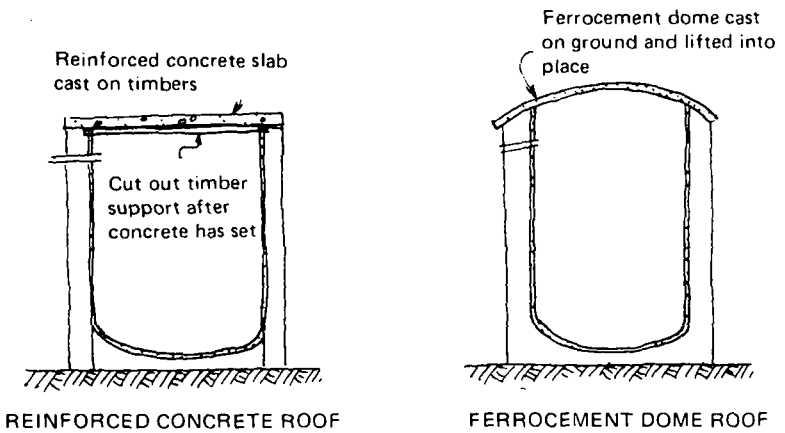
Fig.37 Ferrocement-lined adobe tanks
