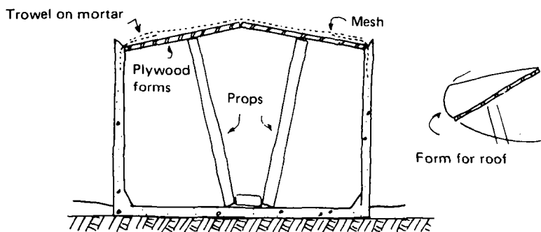
Fig.31 Constructing the roof
