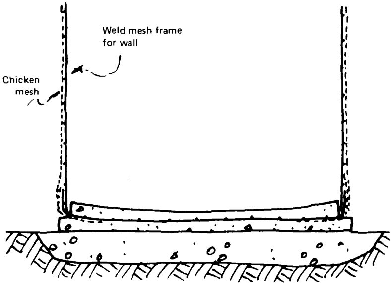
Fig.34 Erecting the wall reinforcement
