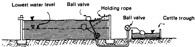
Fig.13 Ball valves for cattle watering
