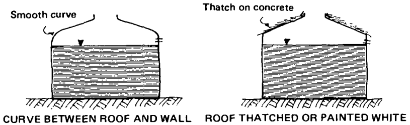
Fig.11 Roofs for tanks less than 5m diameter
