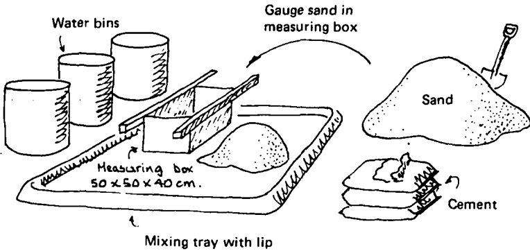
Fig.15 Mixing the mortar by hand
