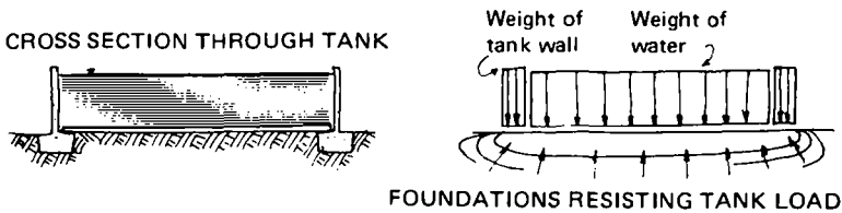
Fig. 6 Foundation of large open tank – walls and floor separate
