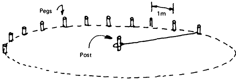
Fig.24 Marking out line of foundation trench
