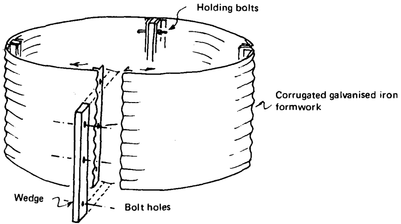
Fig.19 Assembling the formwork
