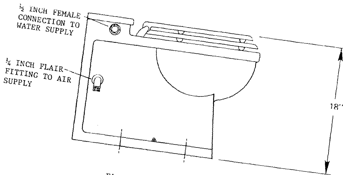
Fig. IX.18. Microphor.
