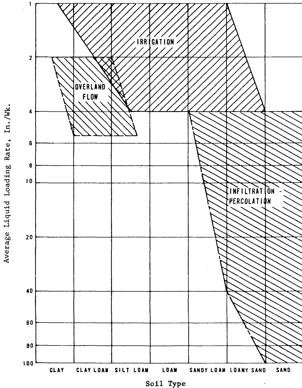
Fig. VIII.3.2. Soil type versus liquid loading rates for different land application approaches.
