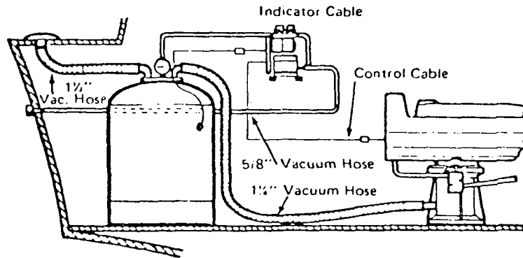
Fig. IX.13. Vacu-Flush.
