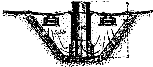
Fig. VI.8. Cross section of Venetian filter-cistern.
