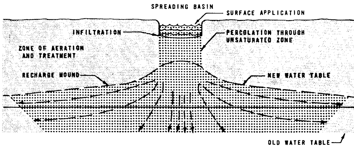
(c) INFILTRATION-PERCOLATION
