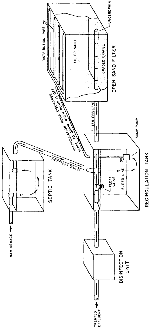
Schematic layout of typical recirculating sand filter sewage treatment system
