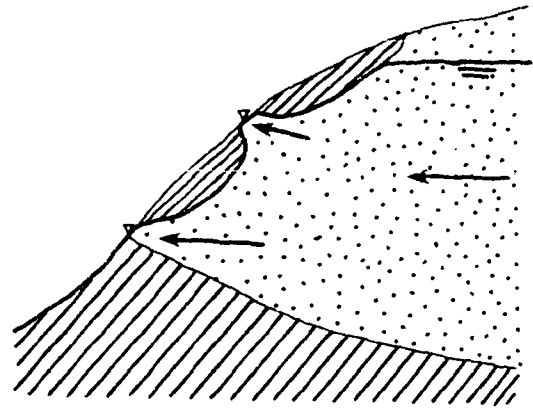
ARTESIAN CONTACT SPRING
