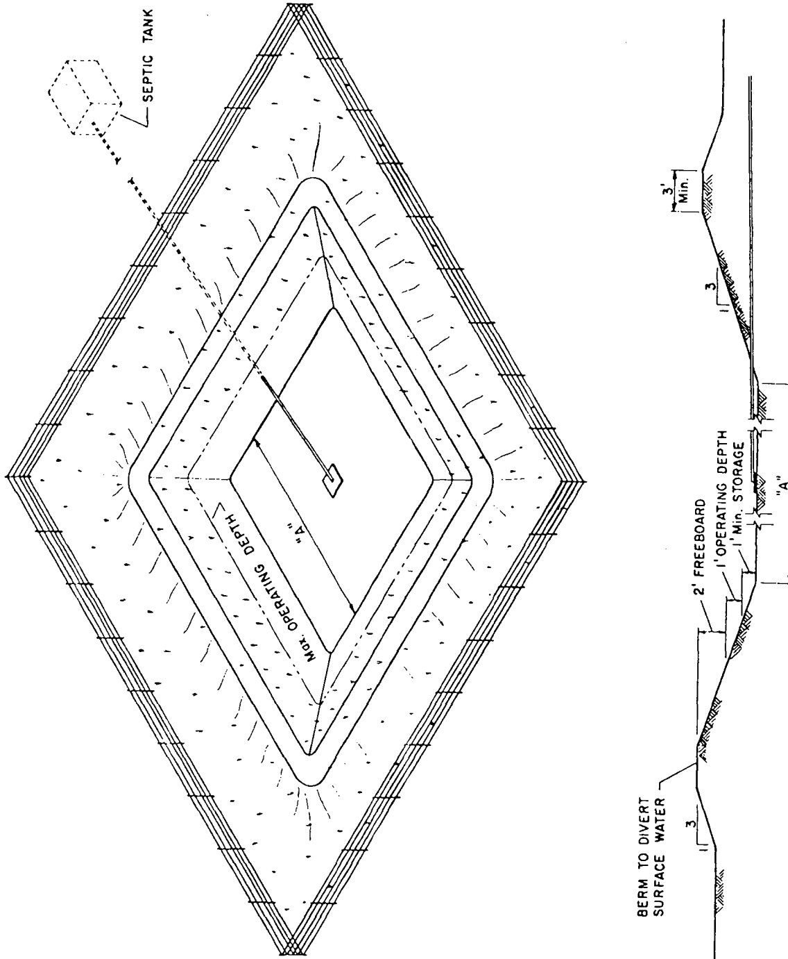
Fig. IX.4. Individual sewage lagoon.
