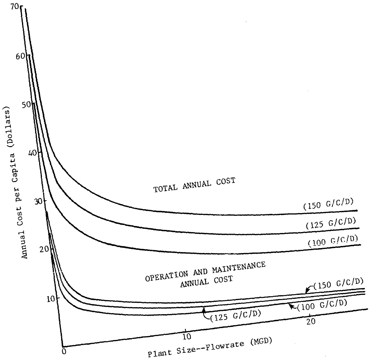
Fig. IX.2. Annual per capita costs according to waste-water treatment plant size.
