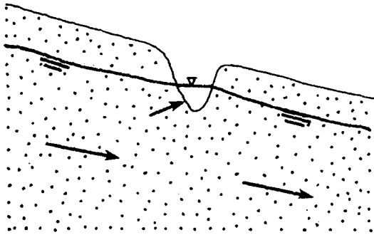
GRAVITY DEPRESSION SPRING
