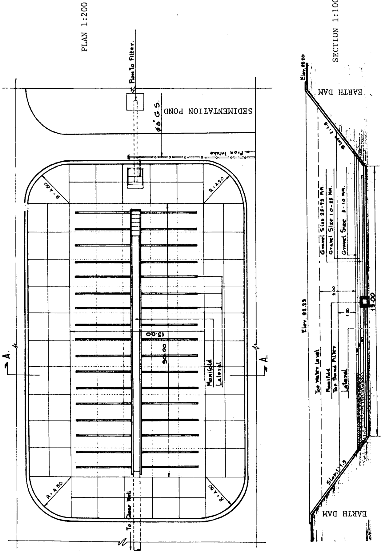
Fig. VII.2.3. Plan and section.
