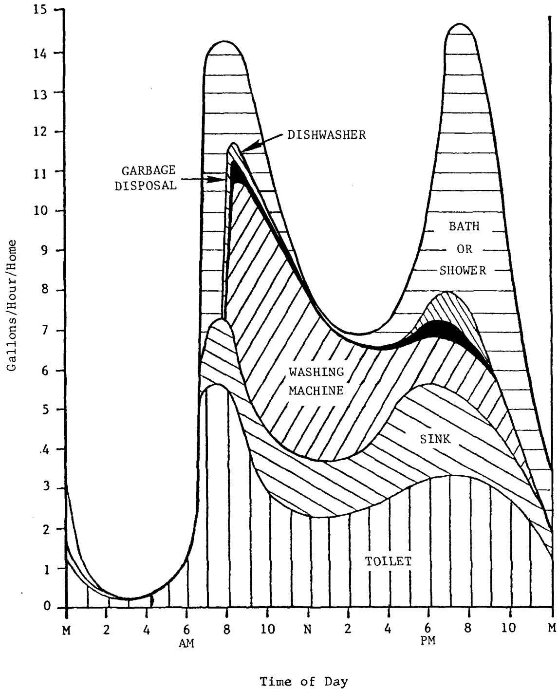
Fig. IX.20. Daily household water use.
