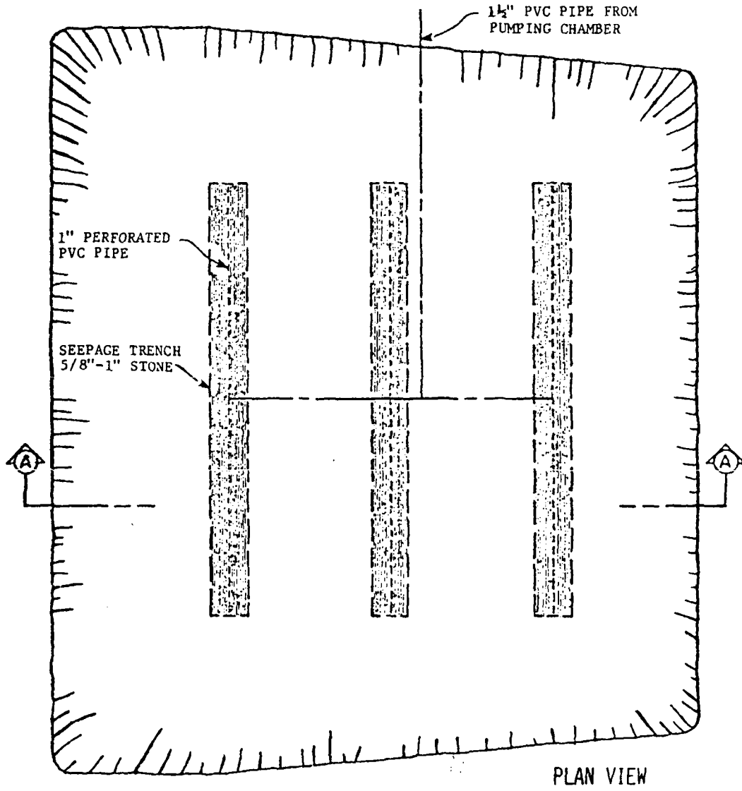
Fig. IX.5. Mound system for a three or four bedroom home.
