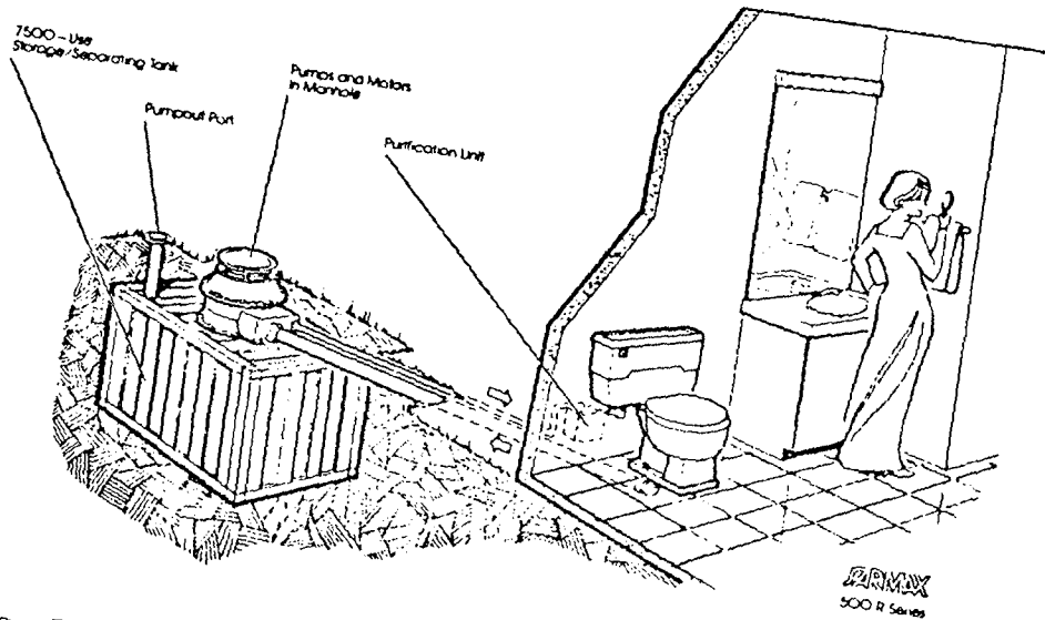
Fig. IX.17. Sarmax 500R Series installed in a home.
