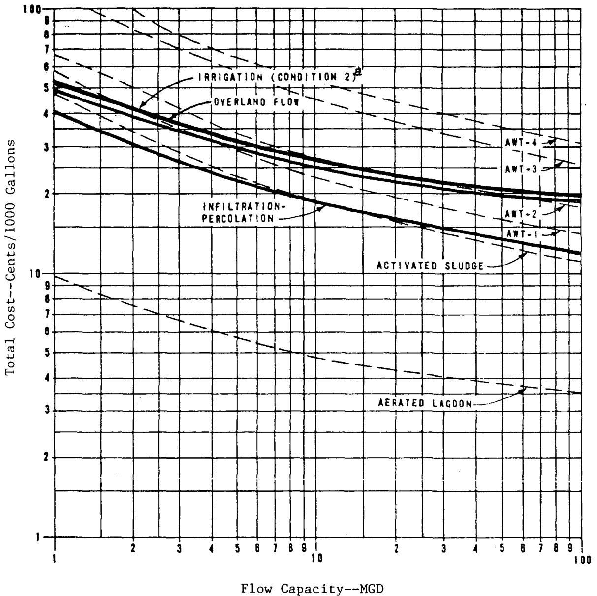
Fig. VIII.3.3. Cost of land applications systems, advanced wastewater treatment (AWT), and other treatment systems.
