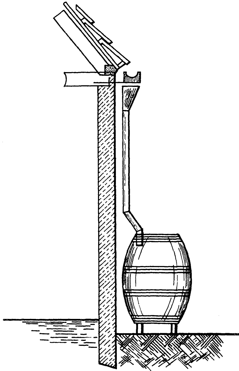
Fig.VII.1.2. Roof catchment.
