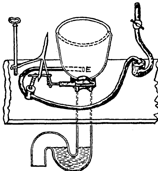
Fig. VI.14. Cumming's valve closet, 1775.
