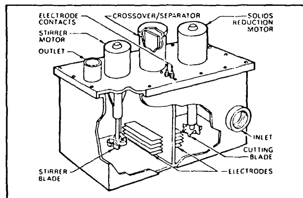
Fig. IX.14. Lectra/San.
