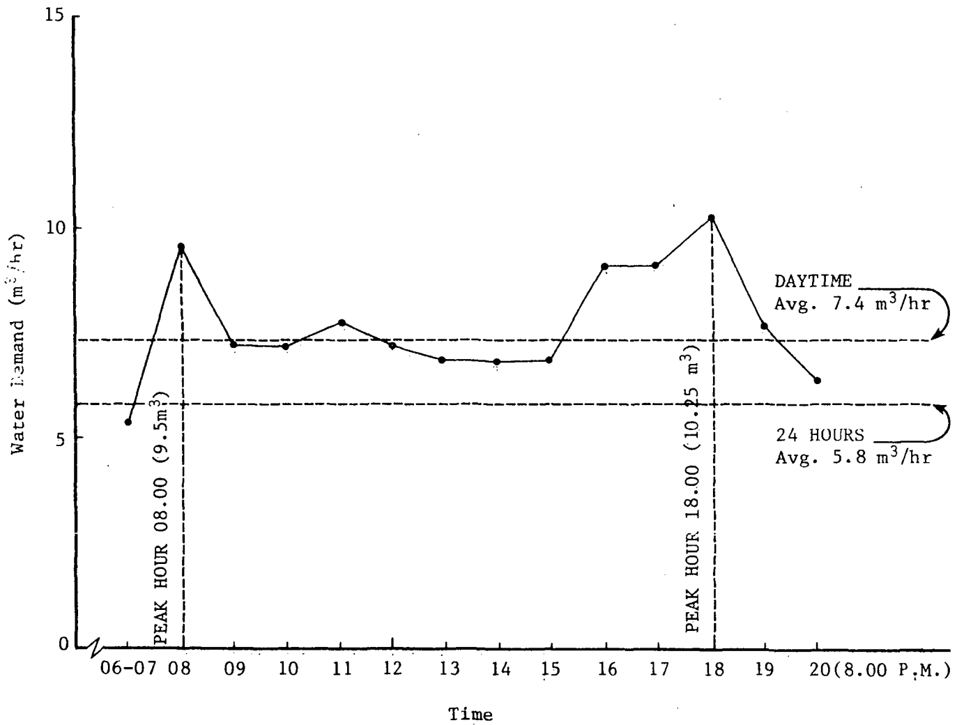
Fig. VII.2.6. Water usage pattern..
