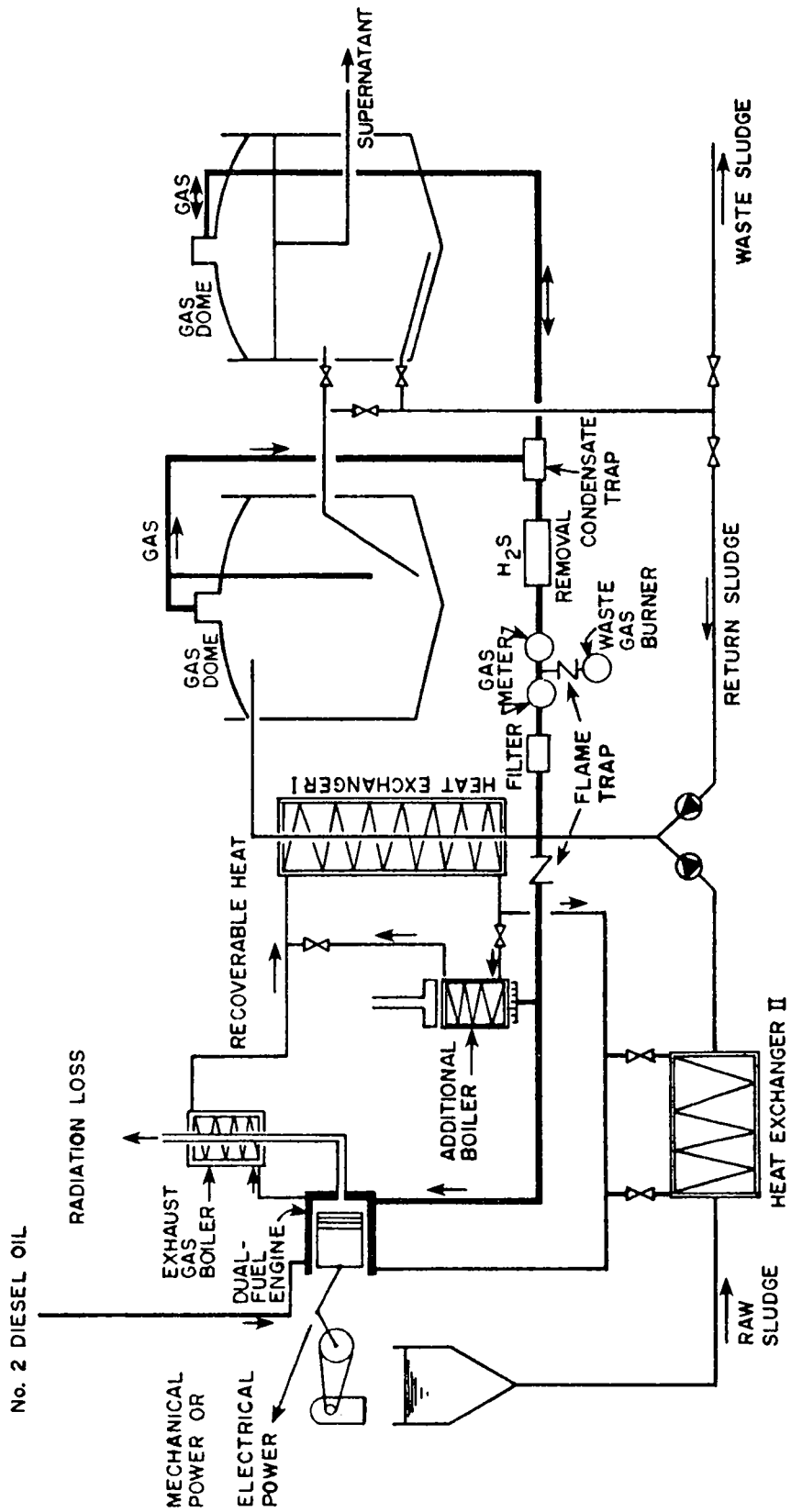
Fig. VIII.1.1.2. Schematic of power and heat generation with dual-fuel engines.
