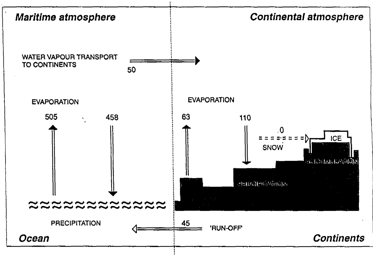
Global water balance estimates (1000 km 3 ) Source: UNESCO, 1978
