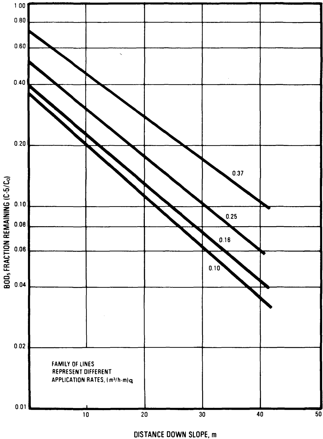
FIGURE 3-2 BOD 5 FRACTION REMAINING VS. DISTANCE DOWN SLOPE WITH PRIMARY EFFLUENT (4)
