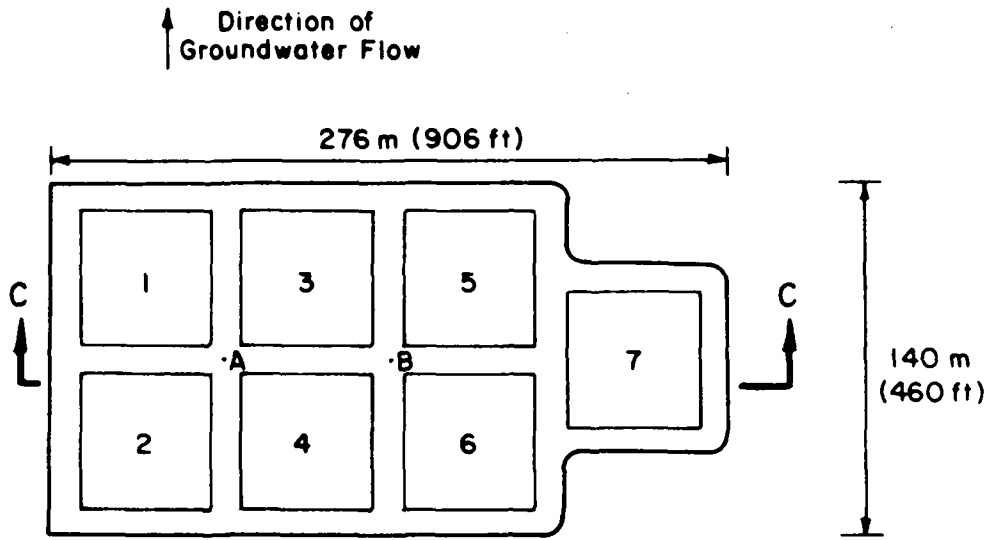
FIGURE 4-1 BASIN LAYOUT FOR EXAMPLE CALCULATION
