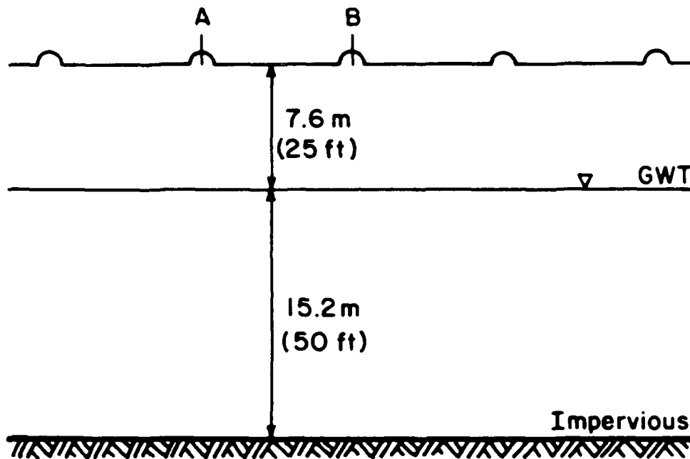
FIGURE 4-2 SUBSURFACE PROFILE SECTION C-C FOR EXAMPLE CALCULATION
