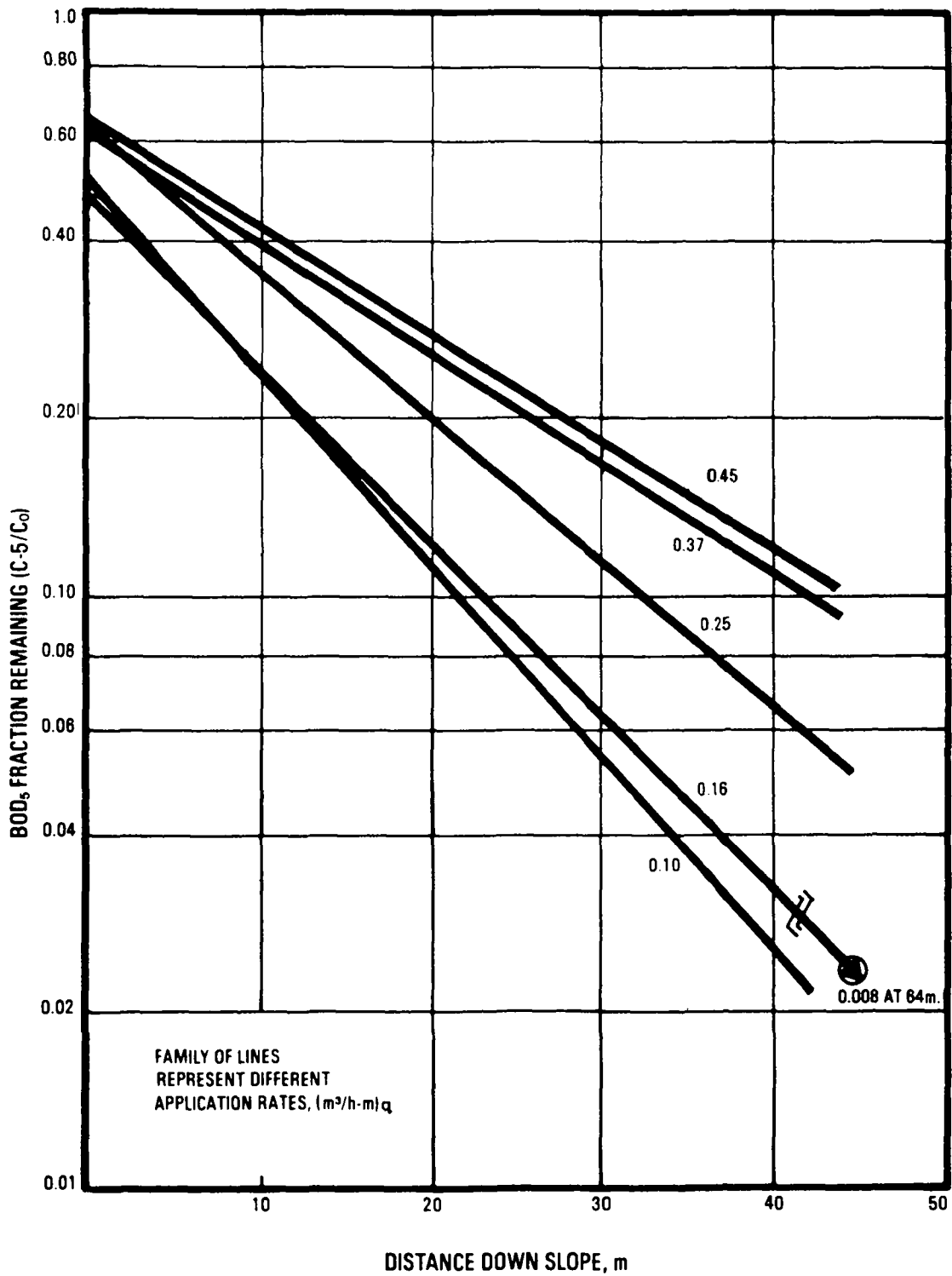
FIGURE 3-1 BOD 5 FRACTION REMAINING VS. DISTANCE DOWN SLOPE WITH SCREENED RAW WASTEWATER (4)
