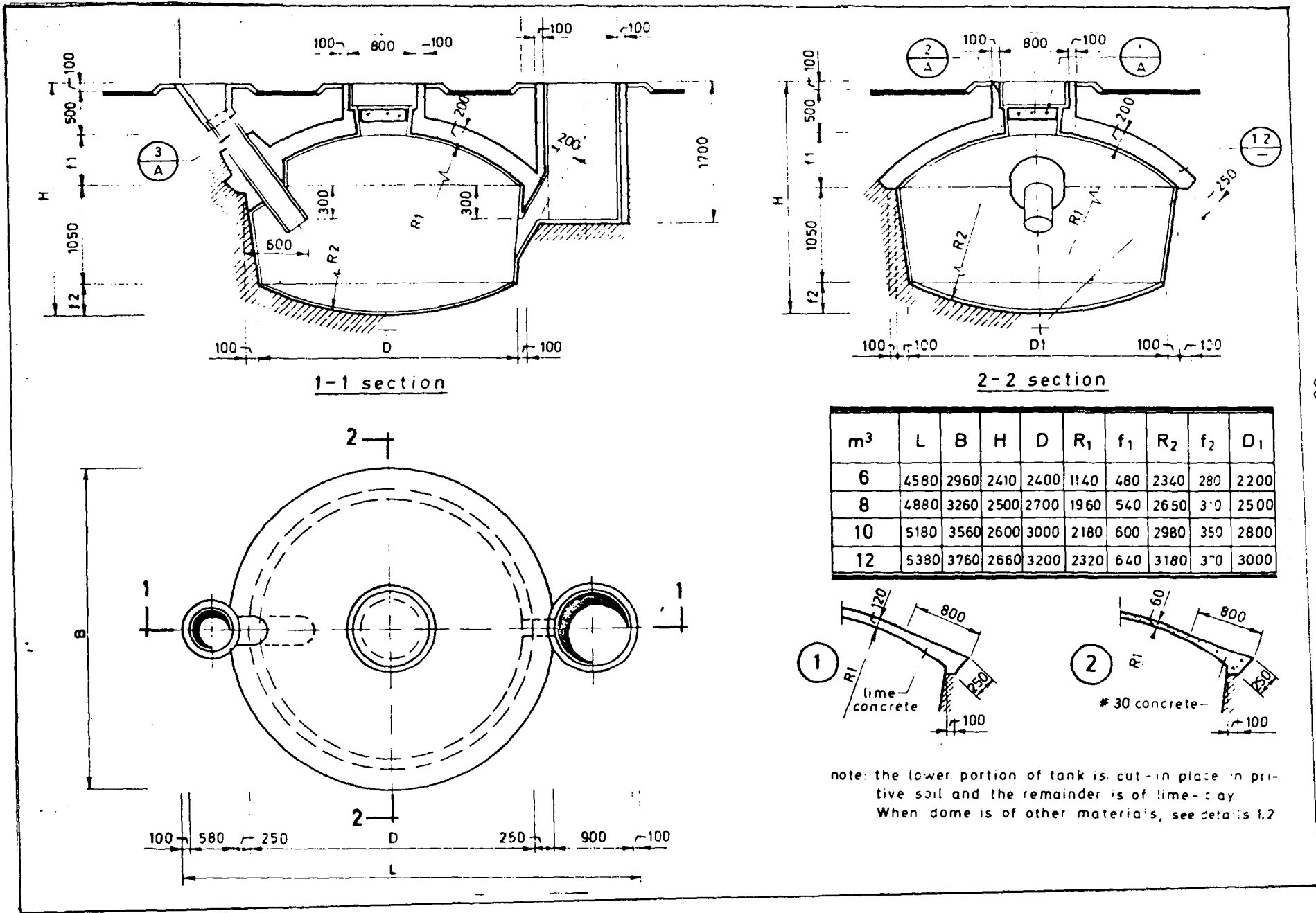
Fig. 25. Design of Cut-in Place Biogas Unit with a Cast Concrete Dome
