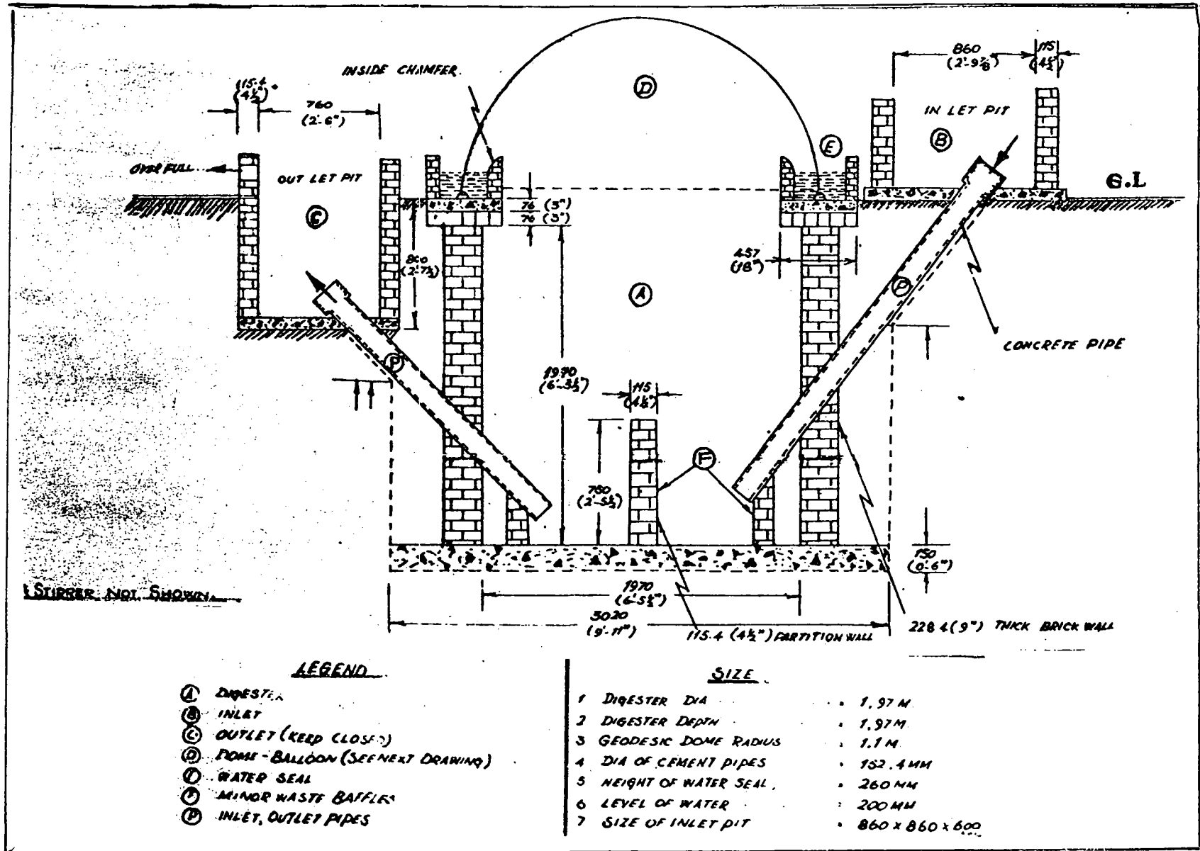
Fig. 14: Jwala Biogas Plant (100 kg) day dung feed)
