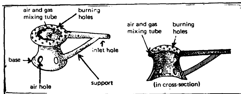
Fig. 50: Long-Arm Burner
