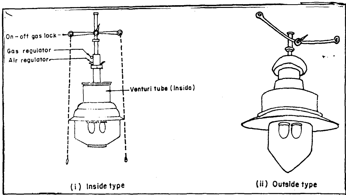
Fig. 55: Double Mantle Lamps (India)
