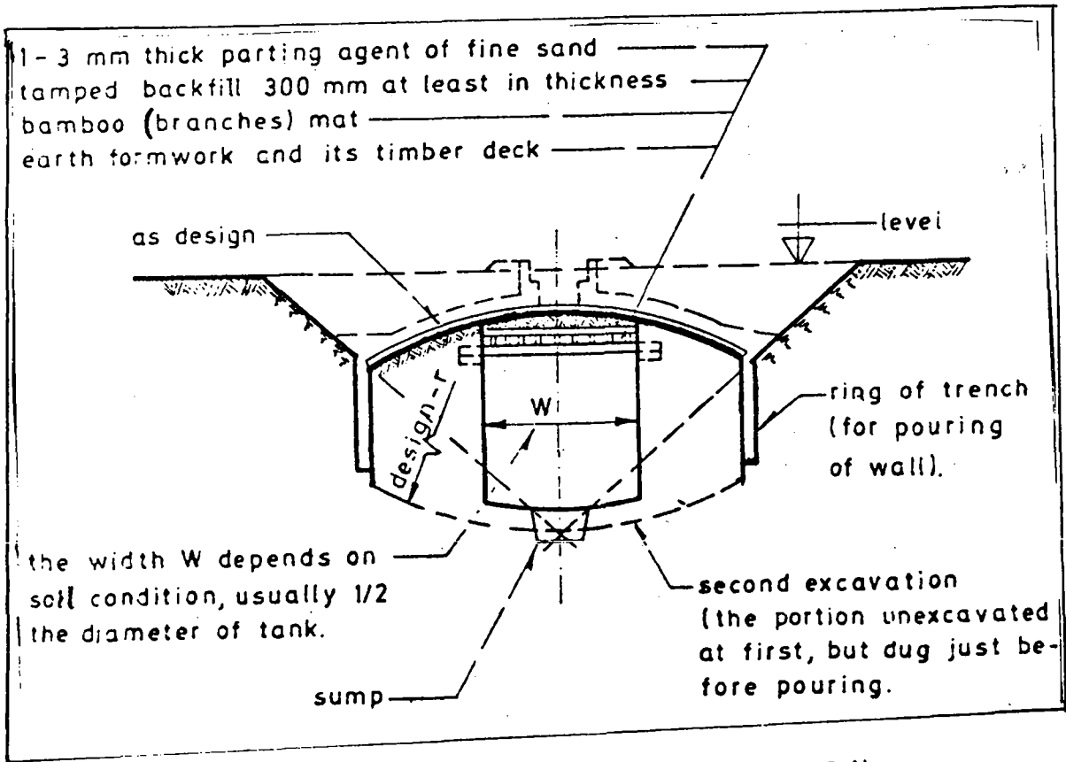
Fig. 17: Design of Cast-in-Place Biogas Unit
