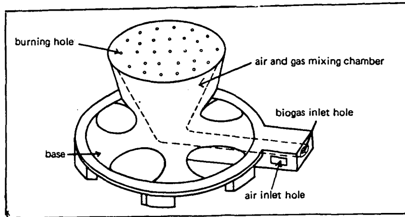
Fig. 46. Shower Head Burner
