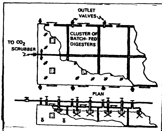
Fig. 35. Biogas Plant Design (Maramba)
