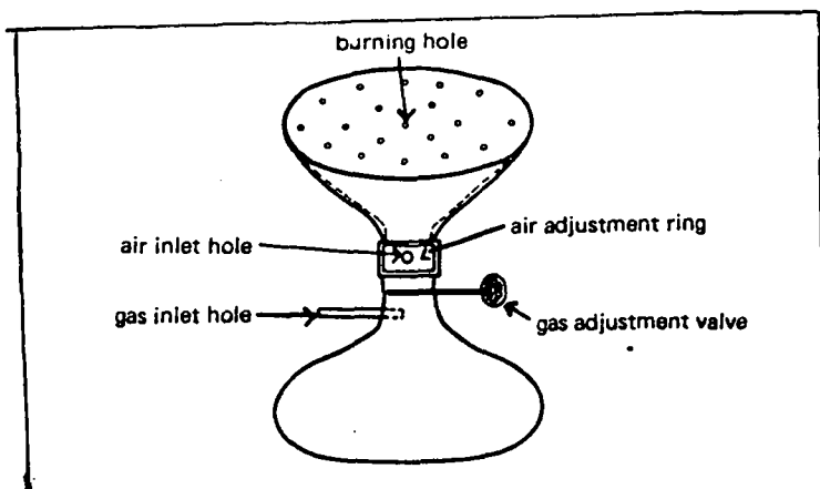
Fig. 48: Hour-Glass Shaped Burner
