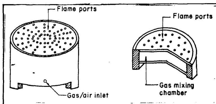
Fig. 49: Drum Burner
