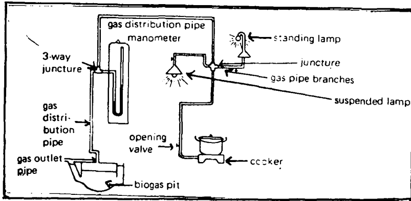
Fig. 58: Plan of Equipment Installation for Biogas Utilization
