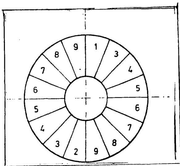
Fig. 18: Casting of Dome According to Numbered Segments
