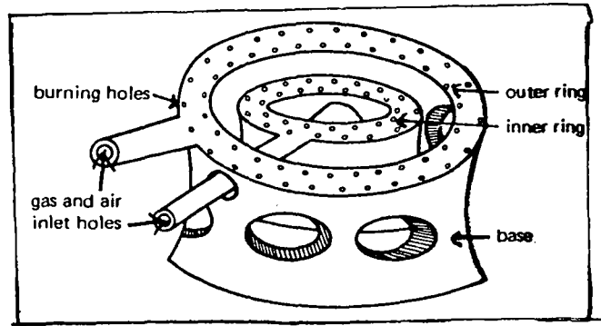
Fig. 51. Double-Ringed Burner
