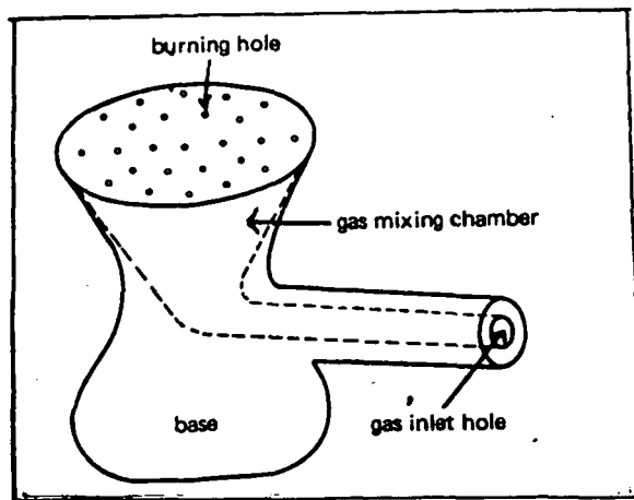
Fig. 47. The L-Shaped Burner
