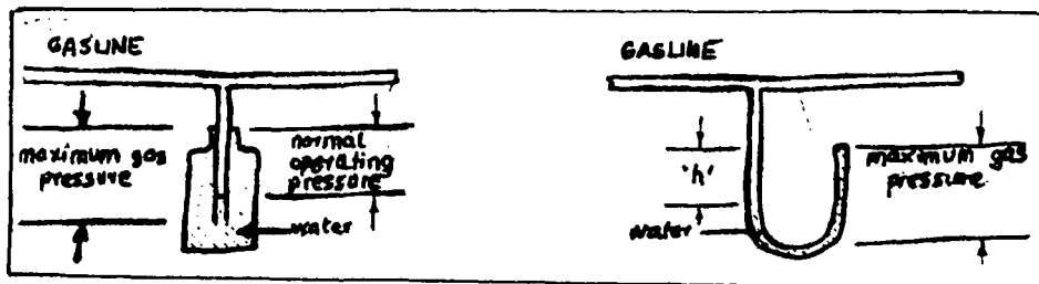
Fig. 33: Water Traps
