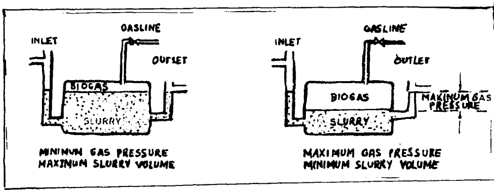
Fig. 32: Pressure in Biogas Bag Digesters
