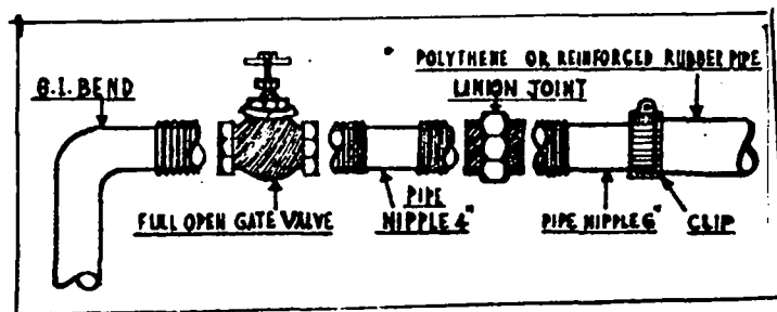
Fig. 8: Pipe Connecting Parts
