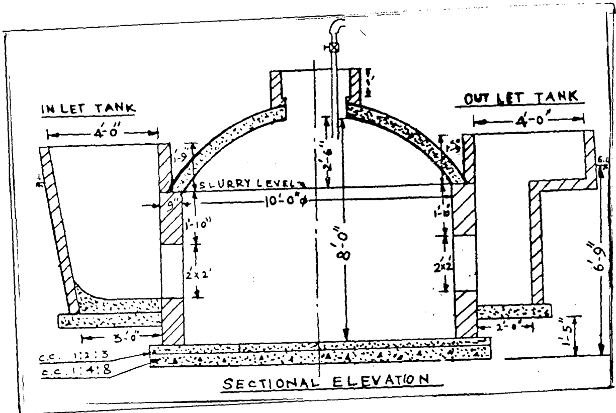
Fig. 26: Janata Biogas Plant
