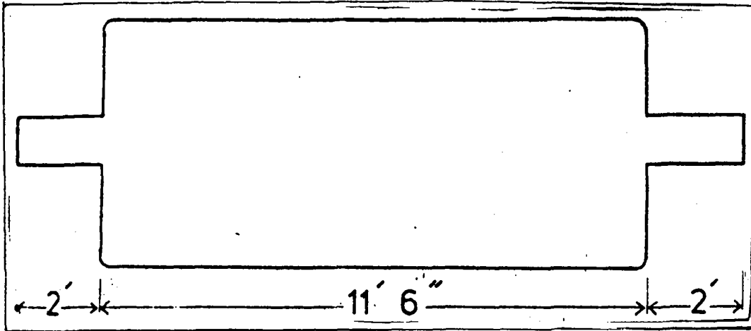
Fig. 30: Plan of the Pit for the Bag Digester
