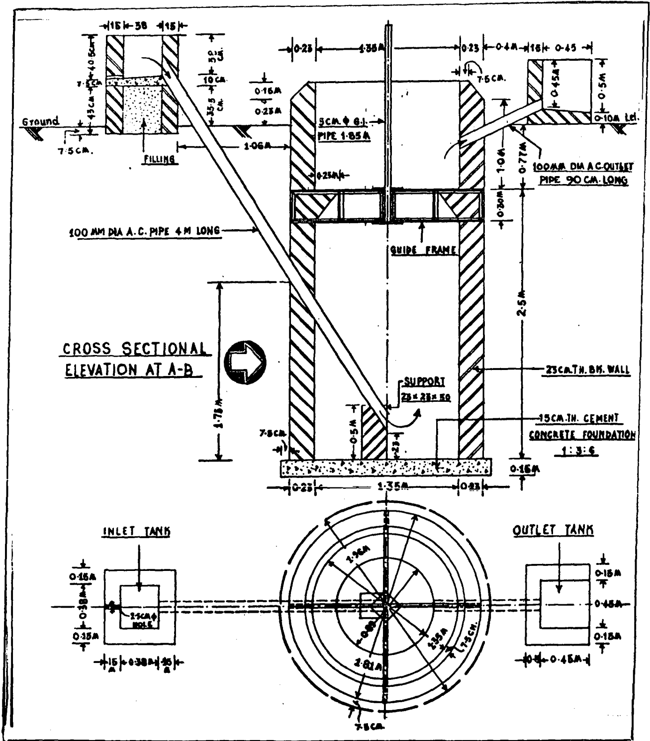
Fig. 4: Plan of 3 cu. m. KVIC plant
