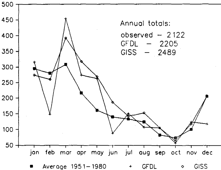
Figure 4. Historical ( 1^*CO_2 ) and GCM-computed ( 2^*CO_2 ) mean monthly precipitations in Mauritius. Sources: Padya (1989, p. 205) for historical values and IIASA's GCM data base for the 2^*CO_2 values.
