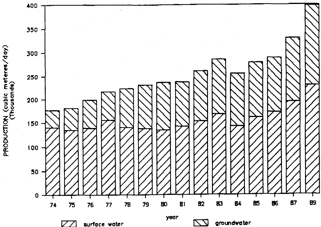
Figure 5. Water production (m 3 /day). Source: Central Water Authority, 1987.
