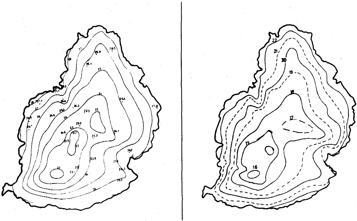
Figure 1. Mean monthly temperatures ( ^{\circ}\text{C} ) in Mauritius in February (a) and August (b). Source: Padya (1989, p. 235).
