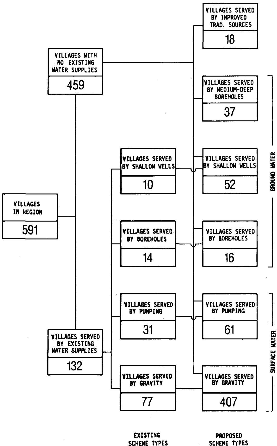
Figure 6.3 - Water Master Plan proposals - village water supply scheme types.
