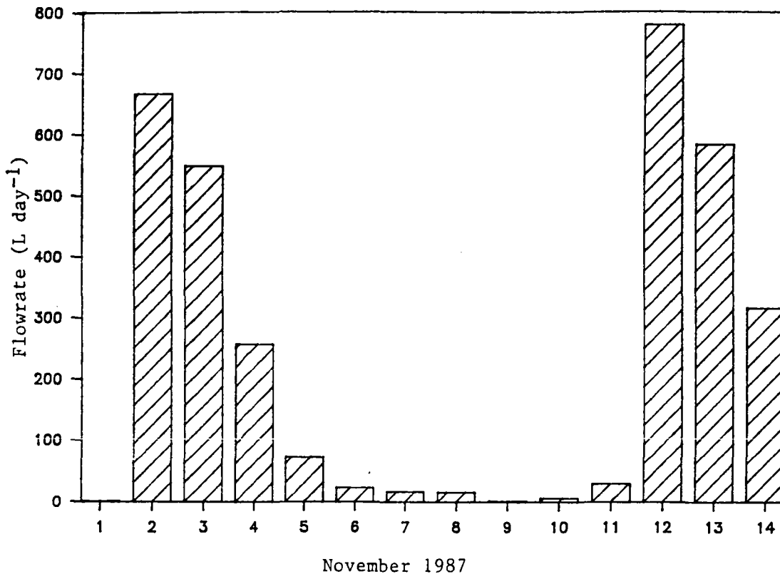
Fig. 3. Mean daily flowrate from atrapaniebla #1 on El Tofo for the first 14 days of November 1987.
