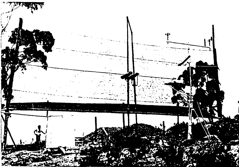
Fig. 2. Atrapaniebla ( 40 \text{ m}^2 fog water collector) on El Tofo plus a meteorological station and droplet measuring equipment.
