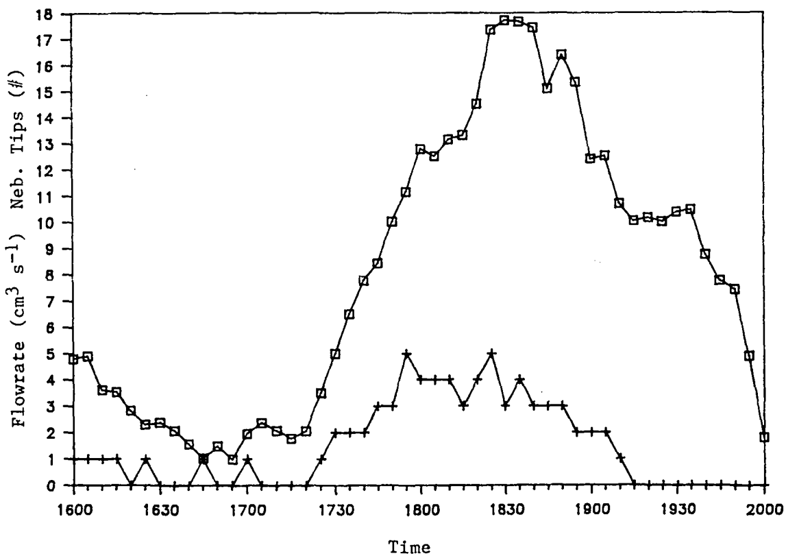
Fig. 4. Comparison of atrapaniebla flowrates (squares) to neblinómetro output (crosses).
