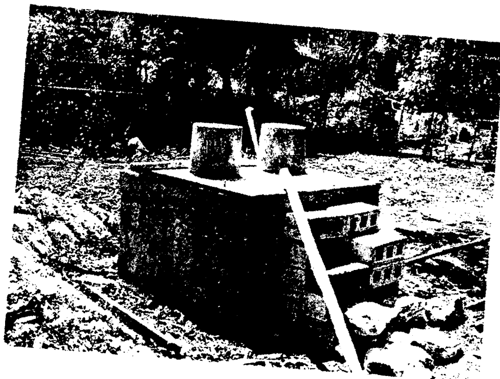
Figure 6. Raised latrine with dual risers.
