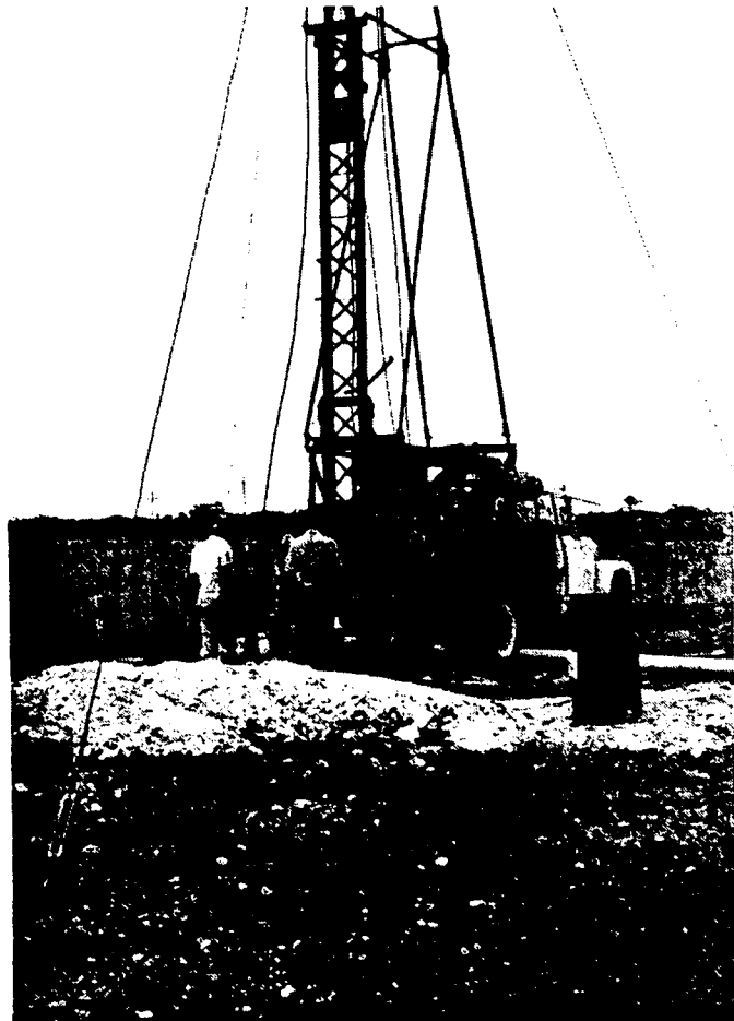
Figure 18. WASA drilling crew with cable tool rig.
