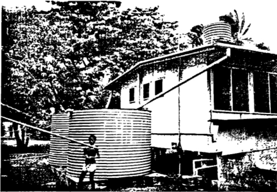
Photo 4. Galvanized steel ground-level and roof tanks.
