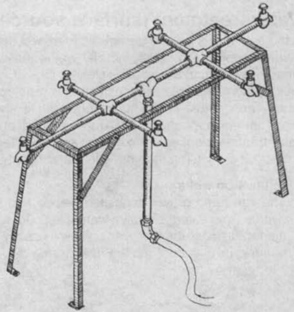
Figure 8: Oxfam water-collection point
