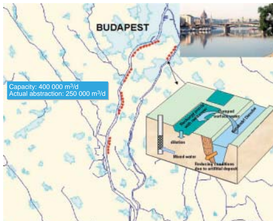
Figure 9. Qualitative improvement of bank filtered water with artificial recharge at Szigetszentmiklós.
