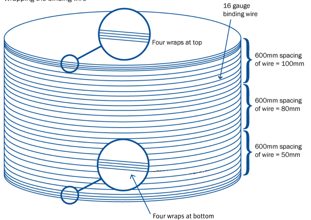
Wrapping the binding wire
