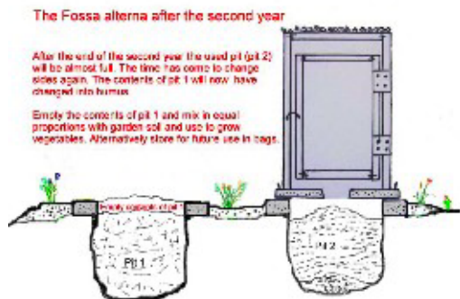
Fig. Fossa Alterna schematic process for second year of use
